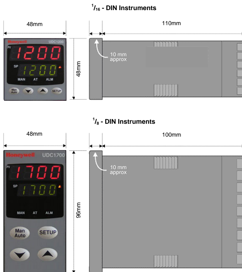
Figure 1. Main dimensions
